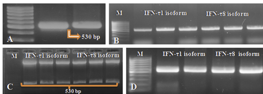
Fig. 2. PCR amplified products of both isoforms from cloning vector using F and R primers having Nco1 and Xho1 restriction sites, respectively (A). Screening of recombinant colonies for both isoforms from transformed top 10 cells: showing three positive clones each for BulFN-T1 and BulFN-T8 isoform (B). Cross checking of Top 10 cells positive clones by restriction digestion with Nco1 and Xho1 restriction enzymes: showing released product of 530 bp (C). Screening of recombinant colonies for both isoforms from transformed BL21 cells: showing two positive clones for BulFN-T1a2 and BulFN-T8 isoform, respectively (D).
